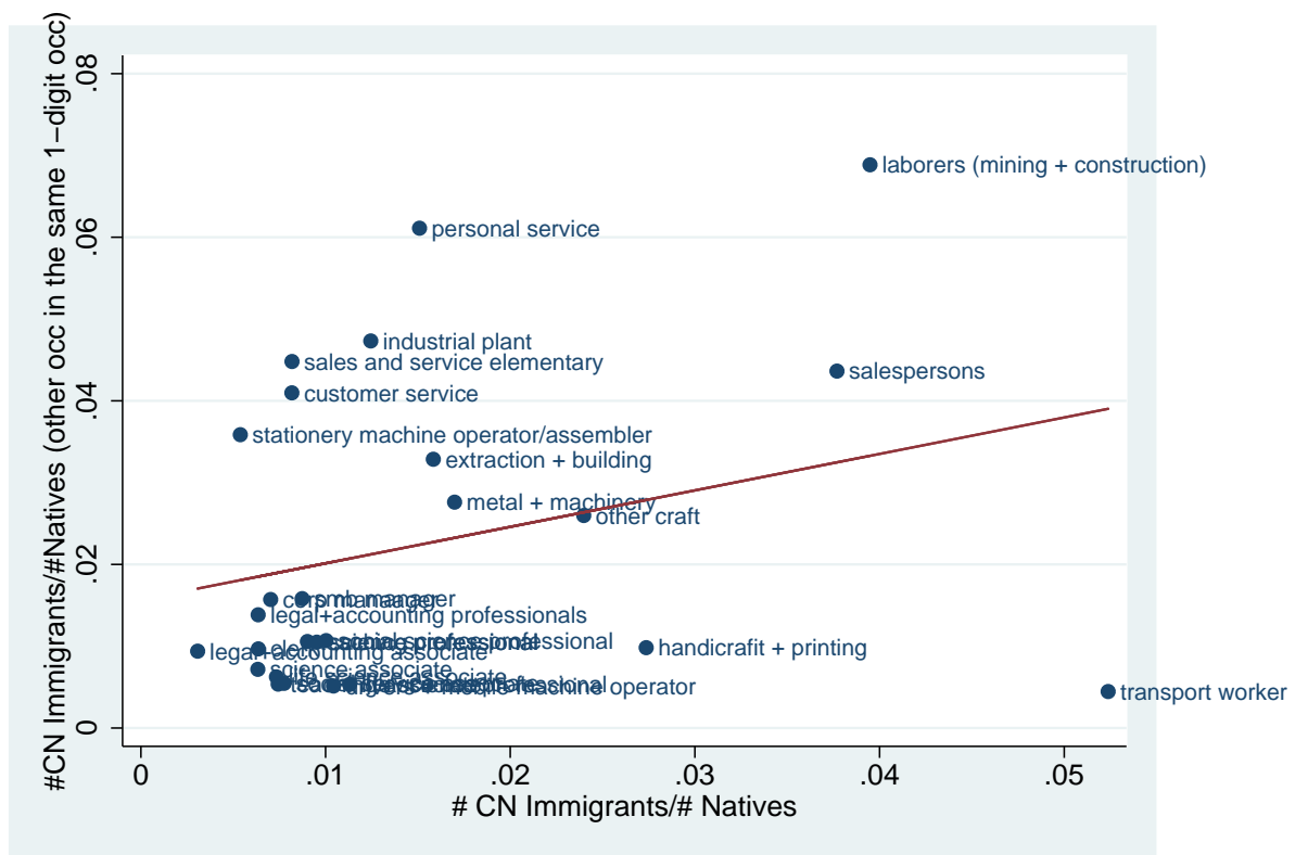
Figure 7: 1996-2001 (Ratio of Chinese Immigrants to Natives in Other Occupations within the same 1-digit Occupation Group) against (Ratio of Chinese Immigrants to Natives) across 3-digit occupations
